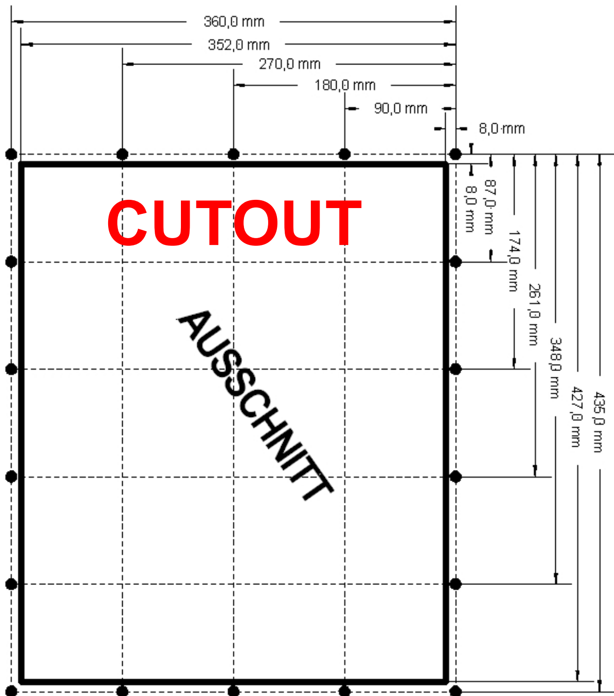
Front Panel Cutout Monitor 17 " Hole = 6.5 mm
